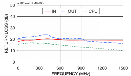
Z30-16-5-75 RETURN LOSS
