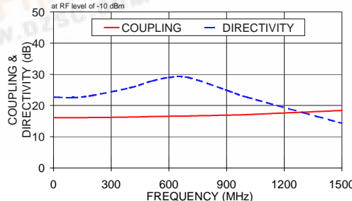
Z30-16-5-75 COUPLING & DIRECTIVITY
