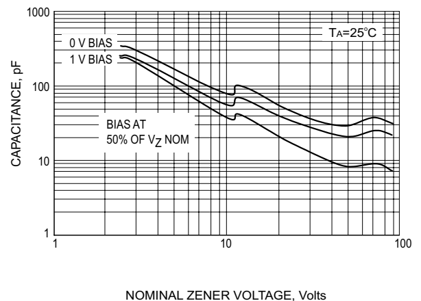
TYPICAL CAPACITANCE
