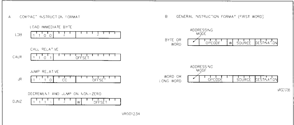
Figure 3-7. Instruction Formats
