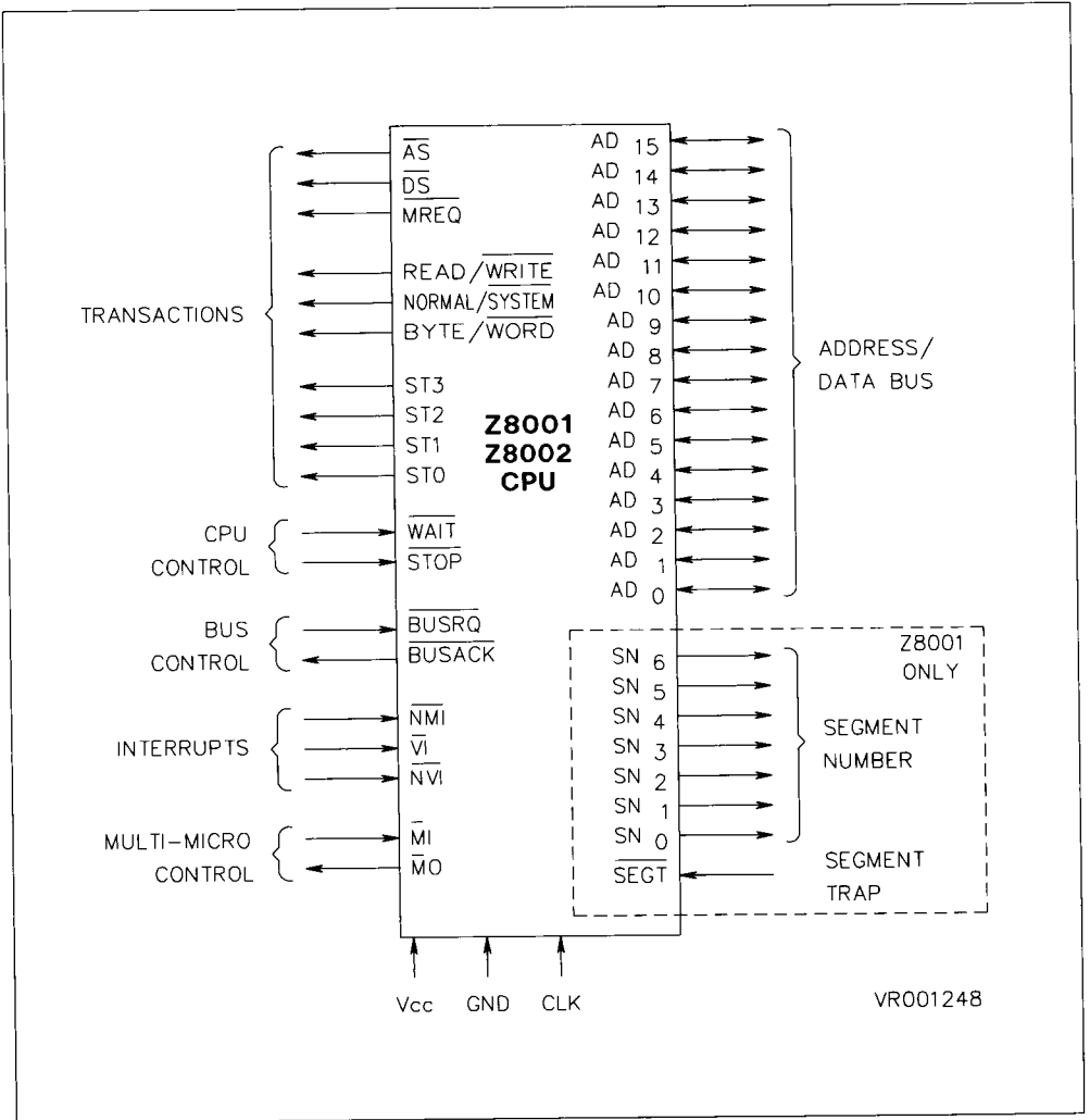
Figure 2-4. Pin Functions
