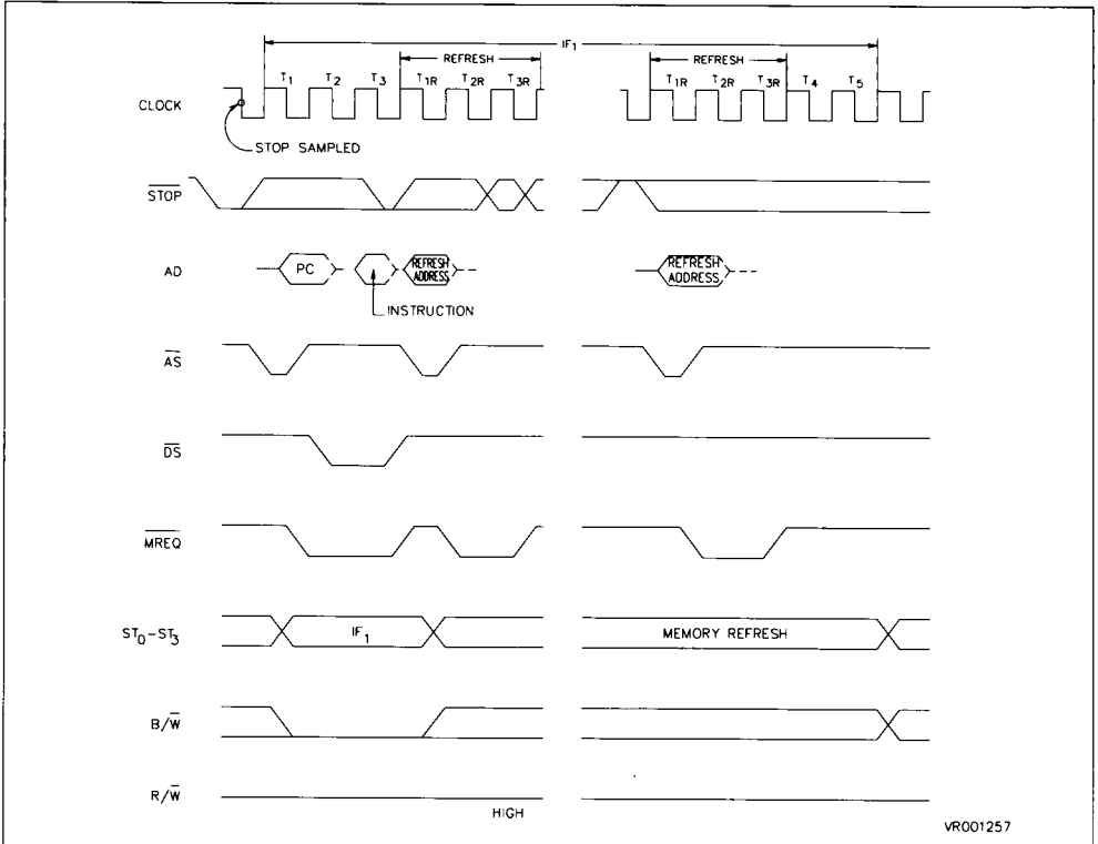
Figure 2-13. Stop Timing
