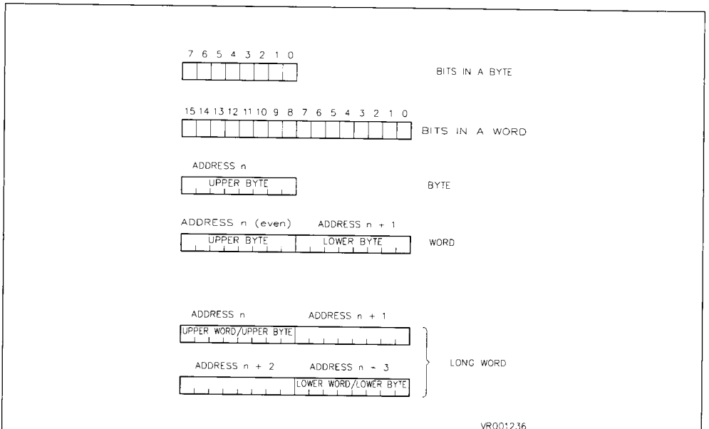
Figure 4-2. Addressable Data Elements
