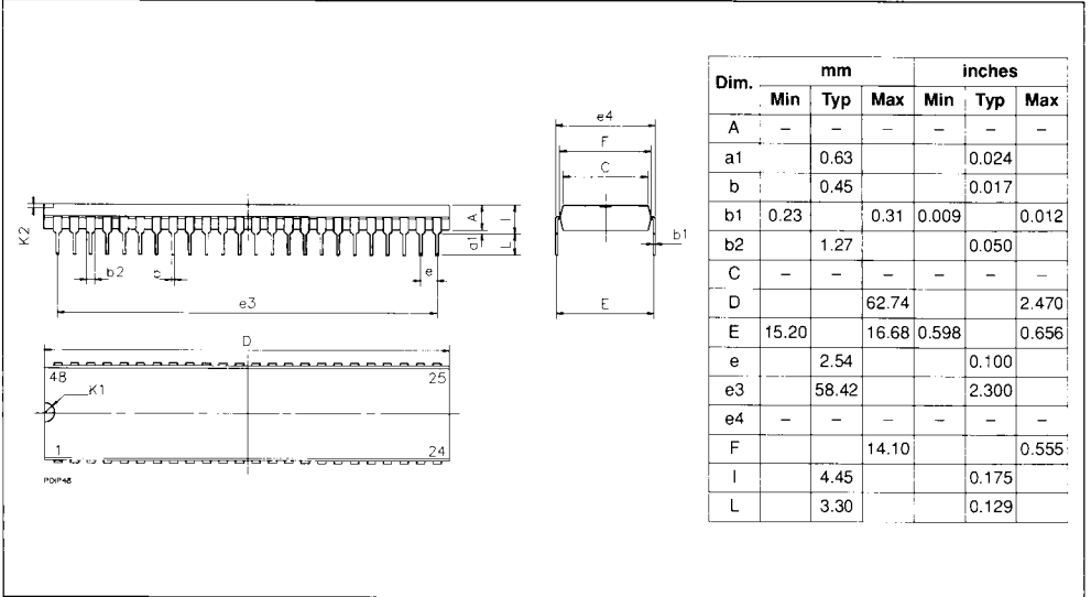
Figure 9-1. PDIP48
