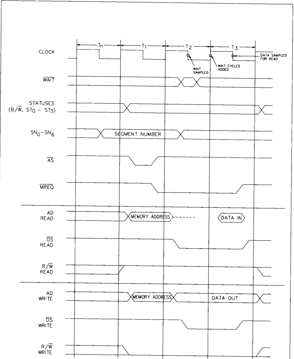
Figure 2-6. Memory Read and Write Transaction
