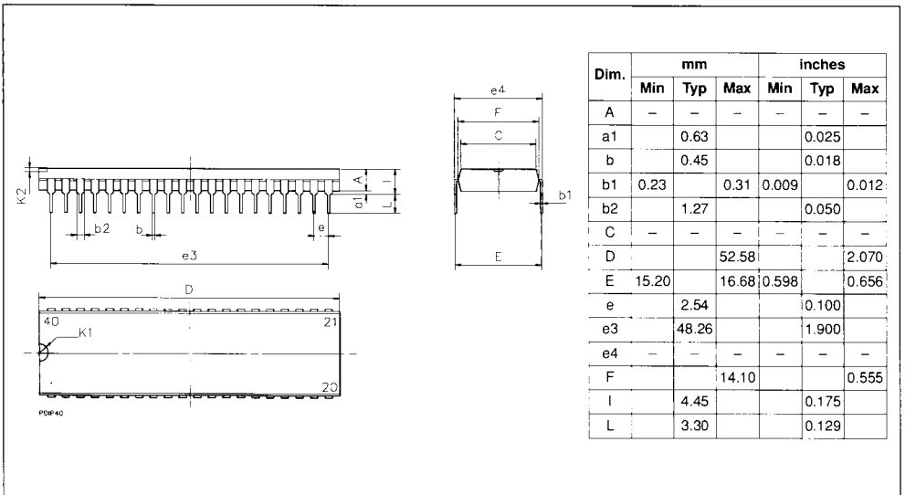
Figure 9-2. PDIP40
