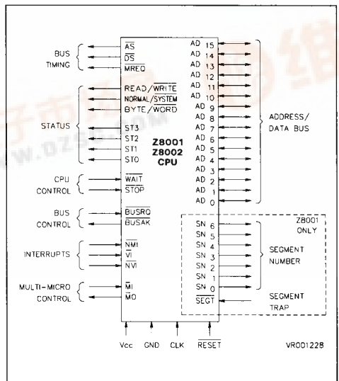
Figure 1-1. Logic Function
