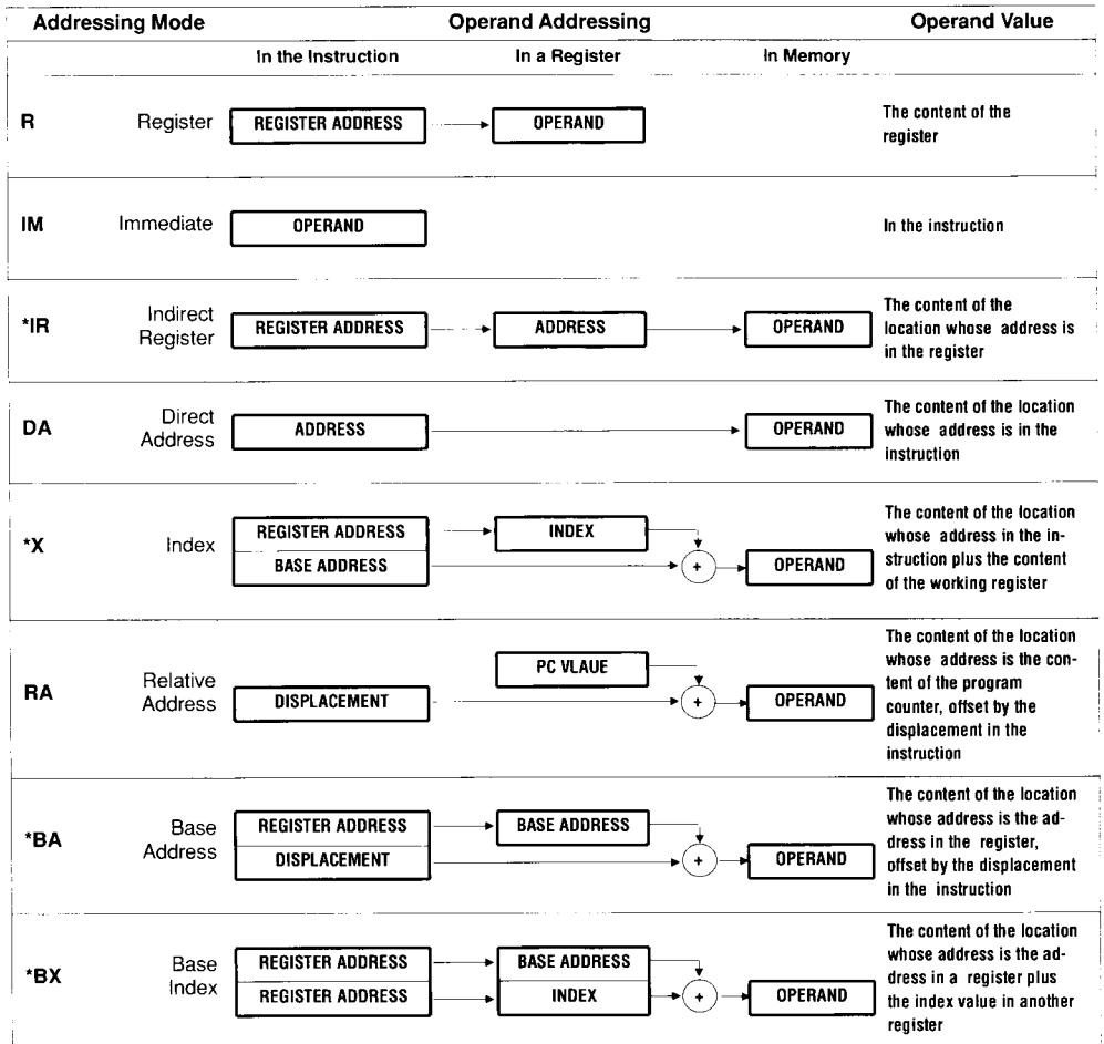
Figure 6-1. Addressing Modes
