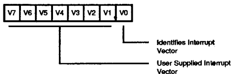
Figure 11. PIO Interrupt Vector Word
