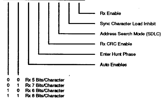
Figure 21. SIO Write Registers
