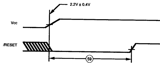
Figure 49. Reset on Power-up (Applies only for Z84C13/C15) (See Table B)
