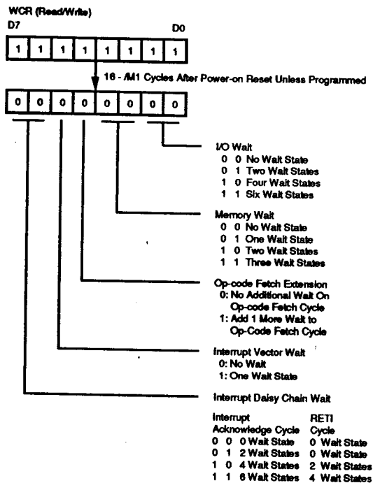
Figure 27. Wait State Control Register
