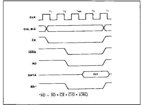
Figure 12 : Read Cycle Timing.
