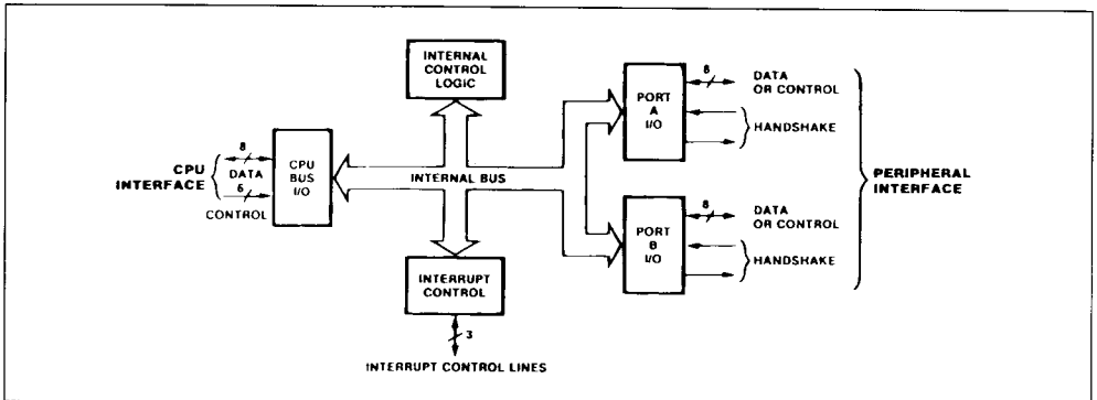
Figure 3 : Block Diagram.
