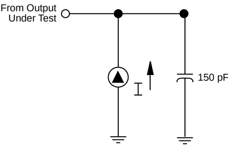
Figure 7. Test Load Diagram
