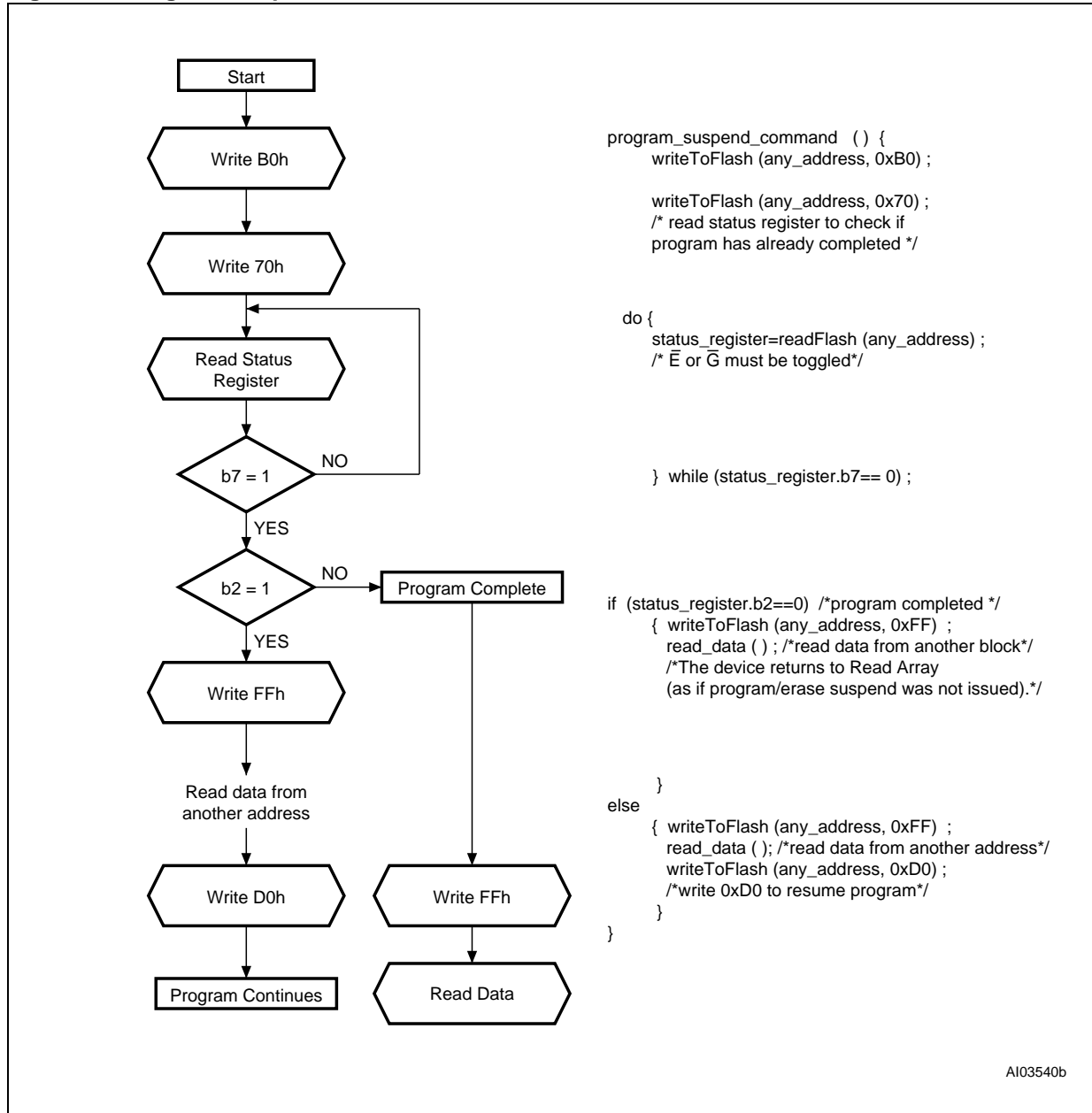
Figure 17. Program Suspend & Resume Flowchart and Pseudo Code
