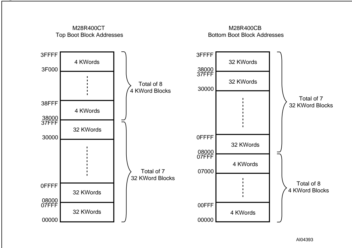
Figure 4. Block Addresses
