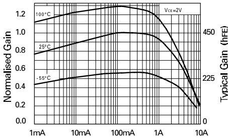
Collector Current
