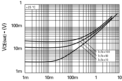
IC - Collector Current (A)
