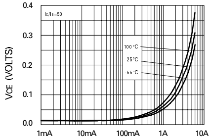
Collector Current
