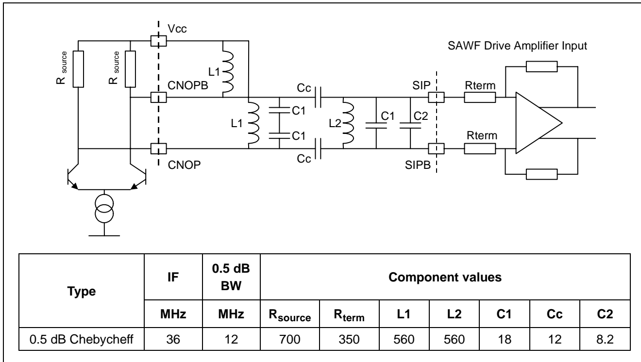
Figure 9 - Interstage Filter
