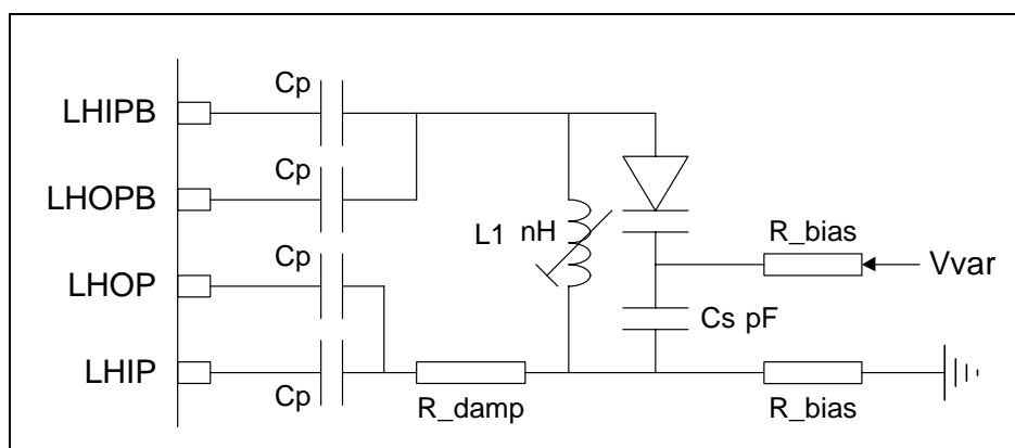
Figure 6 - High Band (UHF) External Tank Circuit
