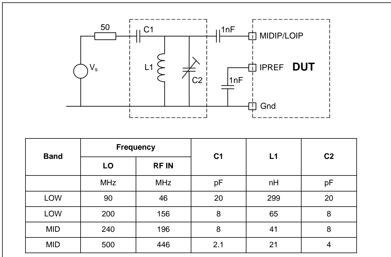
Figure 10 - Noise Figure Measurement Conditions
