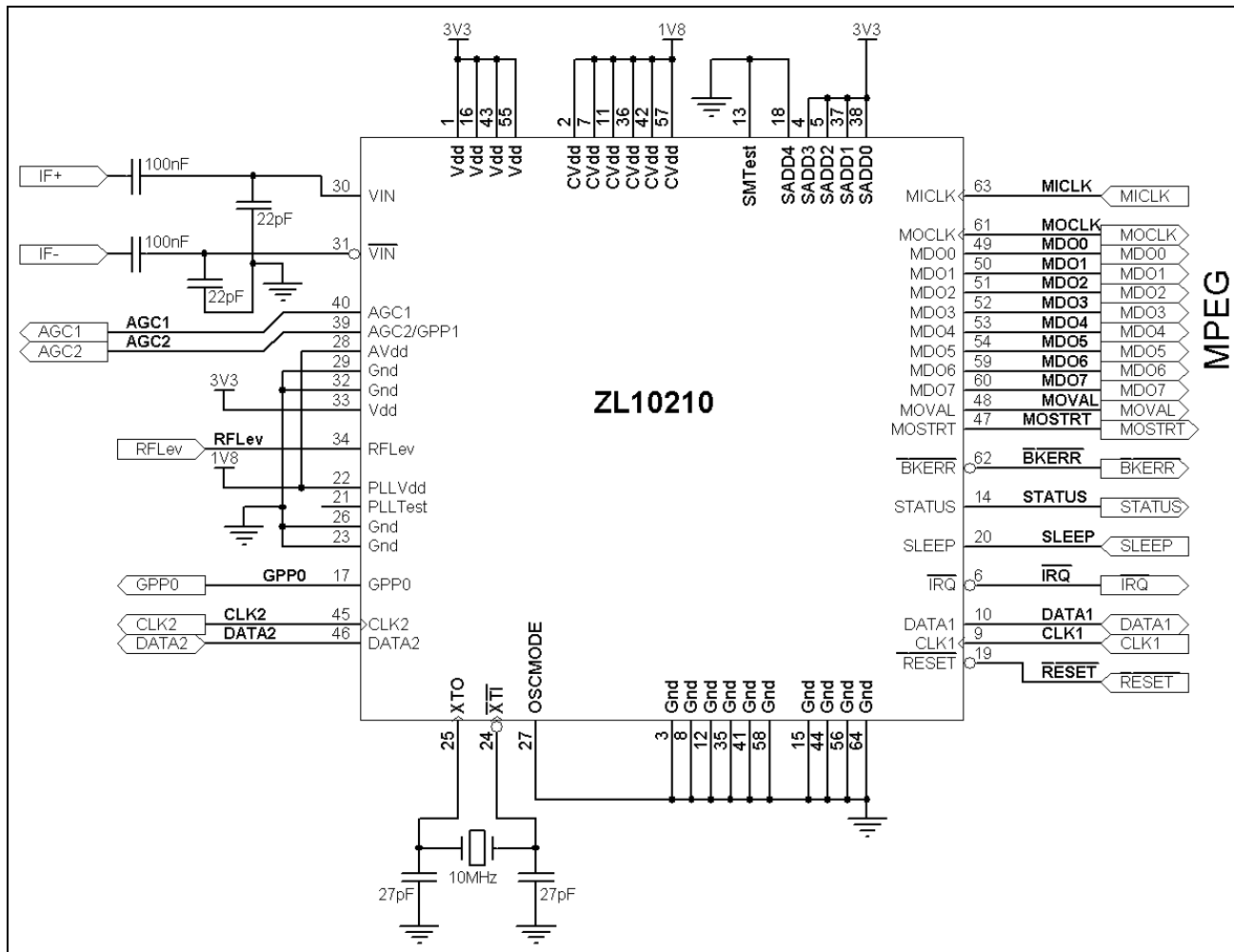
Figure 3 - Typical ZL10210 Application
