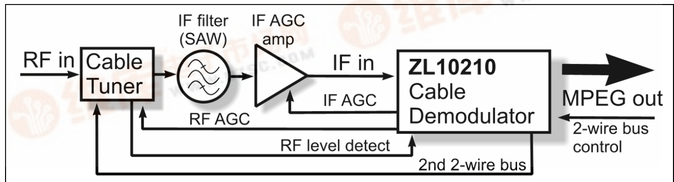
Figure 1 - System Diagram
