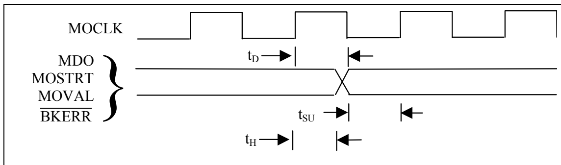
Figure 9 - MPEG Timing - MOCLKINV = 0
