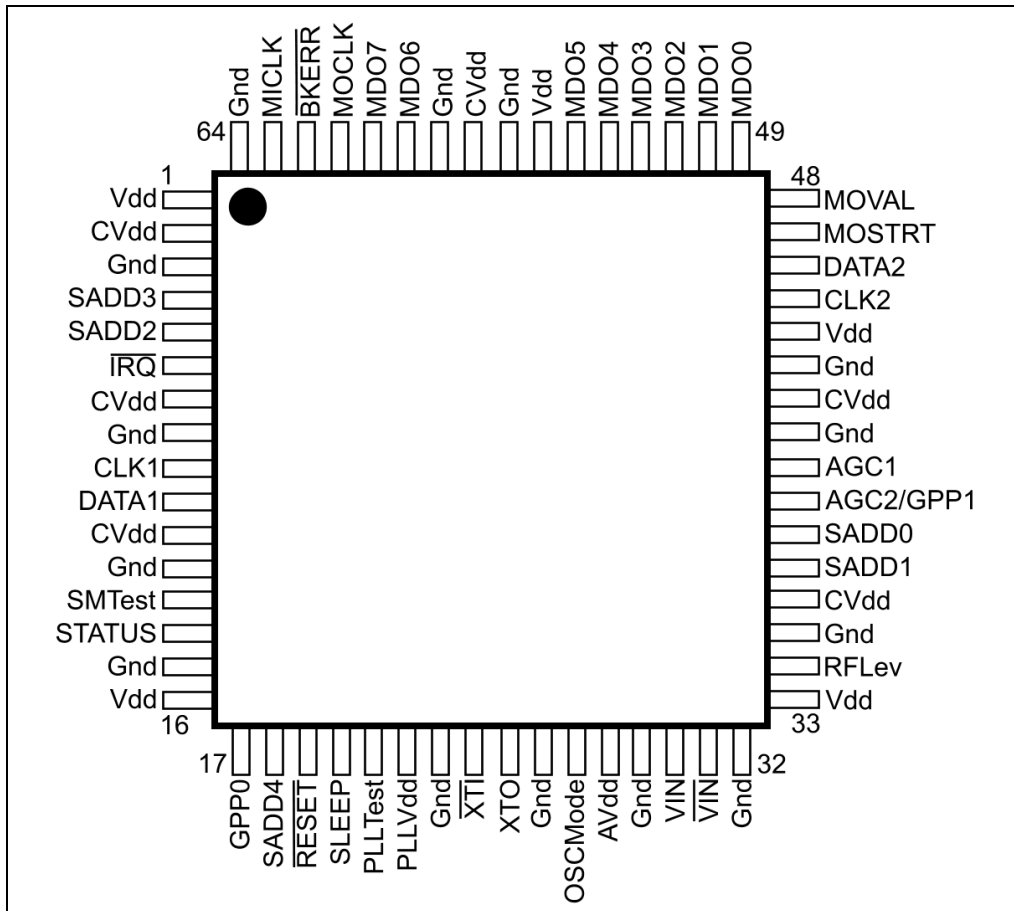
Figure 4 - Pin Outline
