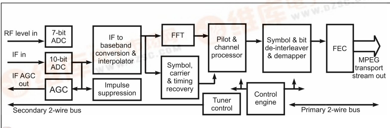
Figure 1 - Block Diagram
