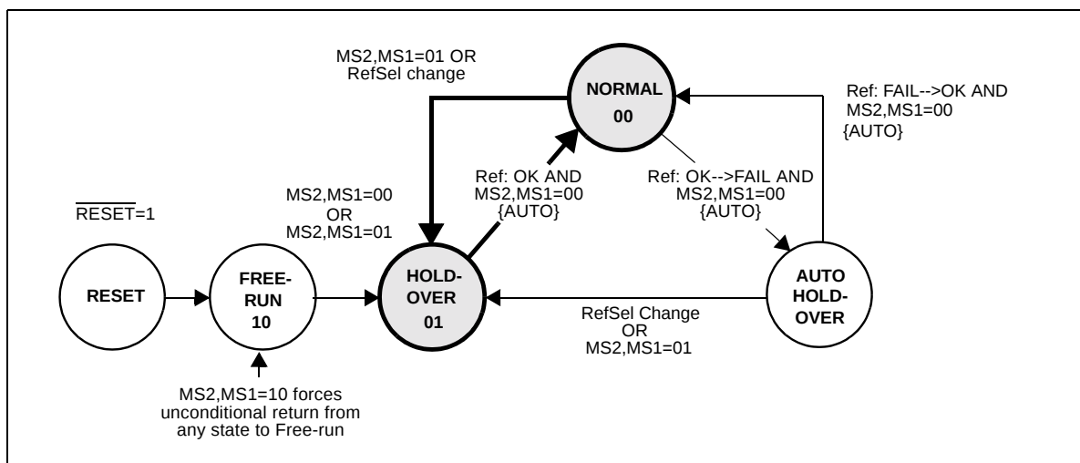
Figure 12 - Manual Reference Switching
