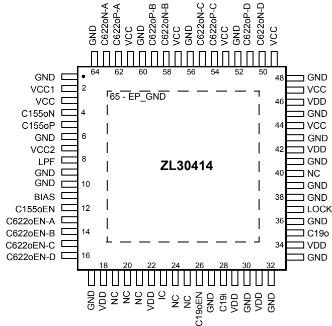
Figure 2 - TQFP 64 pin (Top View)
