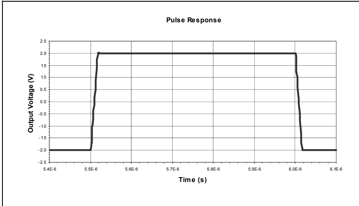
Figure 40 - Pulse Response
