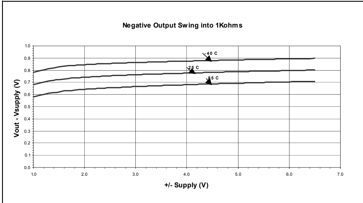
Figure 8 - Negative Output Swing into 1KΩ
