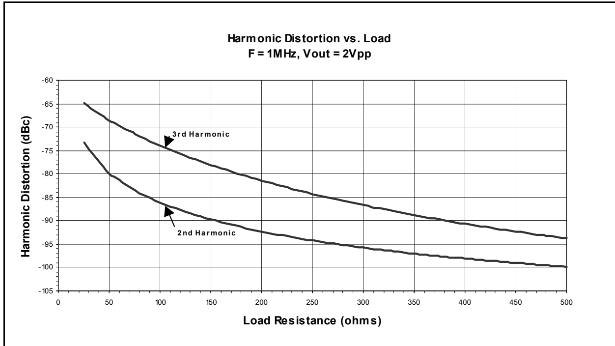
Figure 24 - Harmonic Distortion vs. Load F = 1MHZ, Vout = 2Vpp
