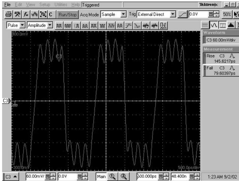
Figure 14 - ZL40800 Single Ended Out @ 5Ghz +2dBm
