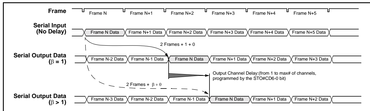
Figure 23 - Data Throughput Delay when Input Channel Delay is Disabled and Output Channel Delay is Enabled for Input Ch0 Switched to Output Ch0
