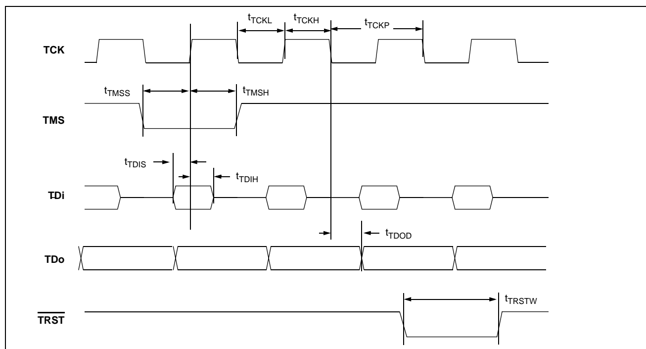
Figure 49 - JTAG Test Port Timing Diagram
