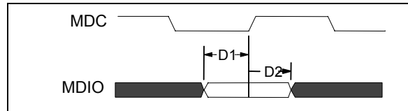
Figure 24 - MDIO Input Setup and Hold Timing
