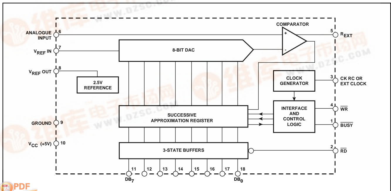
Fig.2 System diagram
