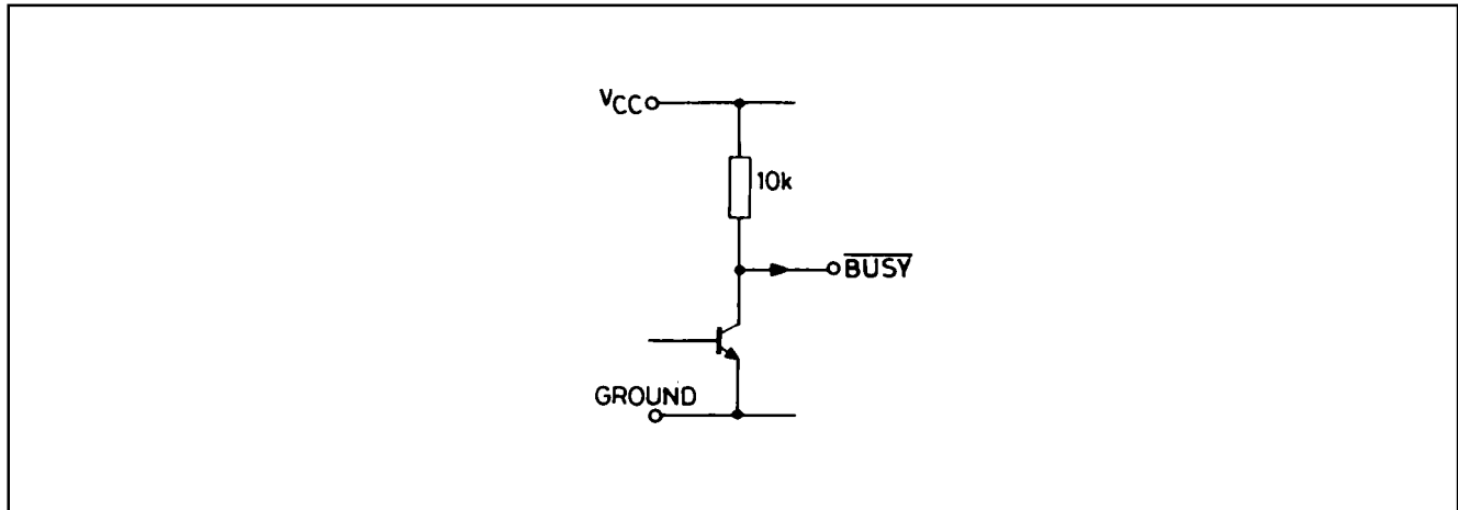
Fig.7 BUSY output
