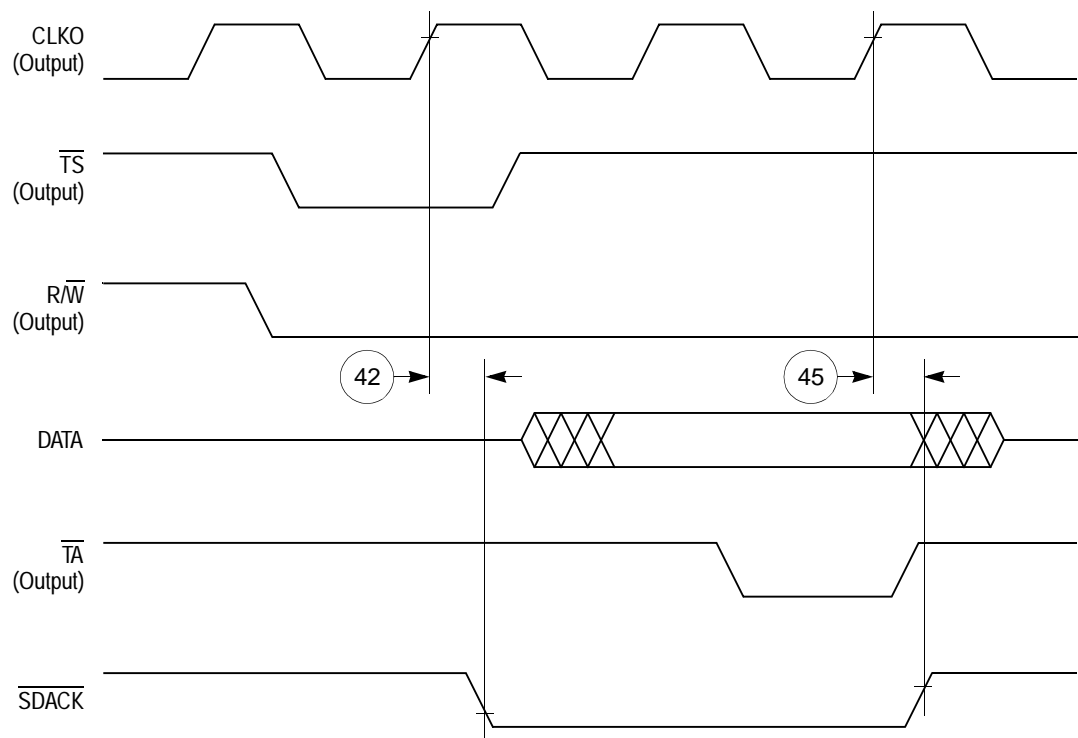
Figure 50. SDACK Timing Diagram—Peripheral Read, Internally-Generated TA
