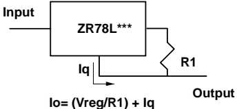
Current Regulator
