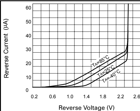
Reverse Characteristics
