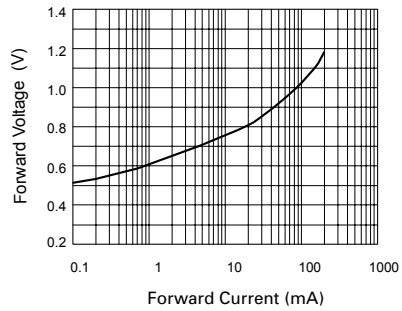
Forward Characteristics
