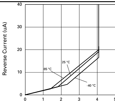
Reverse Characteristics
