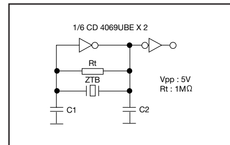
Figure 4) ZTB Test Circuit
