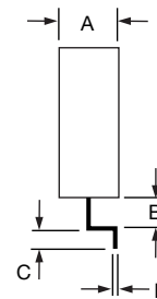
Figure 3) ZTBF (formed lead option) Side views
