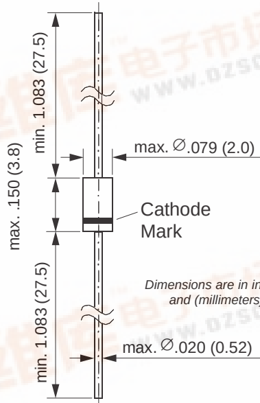
DO-204AH (DO-35 Glass)
