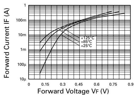
I_F v V_F Characteristics
