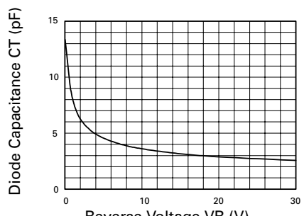
C_T v V_R Characteristics
