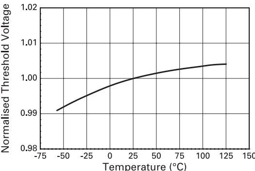
Normalised Threshold Voltage vs Temperature
