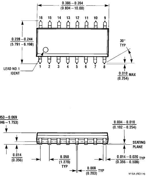
16-Lead (0.150 Wide) Molded Small Outline Package, JEDEC Order Number DS91M047TMA NS Package Number M16A
