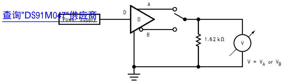
FIGURE 4. Differential Driver DC Open Test Circuit
