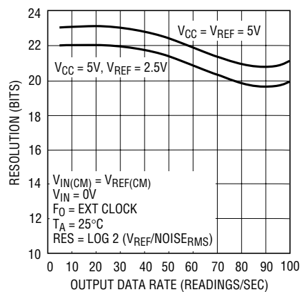
Figure 35. Resolution ( \text{Noise}_{\text{RMS}} \leq 1\text{LSB} ) vs Output Data Rate and Temperature
