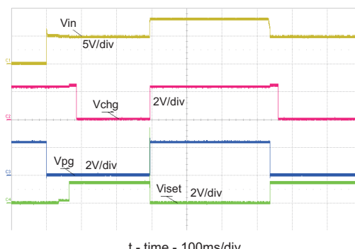
Figure 6. OVP from Normal Power-up Operation - V_{IN} 0V → 5V → 8V → 5V
