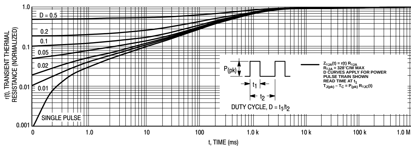
Figure 25. Thermal Response
