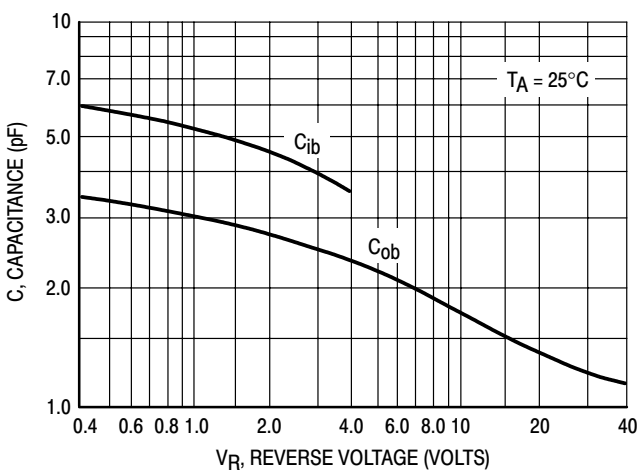
Figure 17. Capacitances
