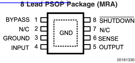
Top View See NS Package Number MRA08A
