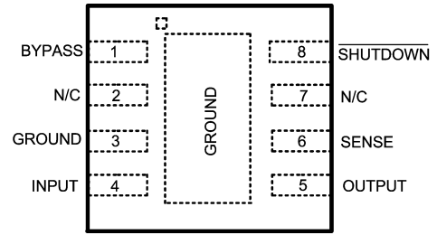
Top View See NS Package Number SDC08A
