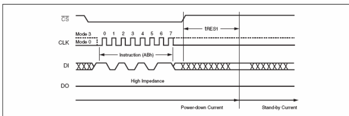
Figure 15. Release Power-down Instruction Sequence
