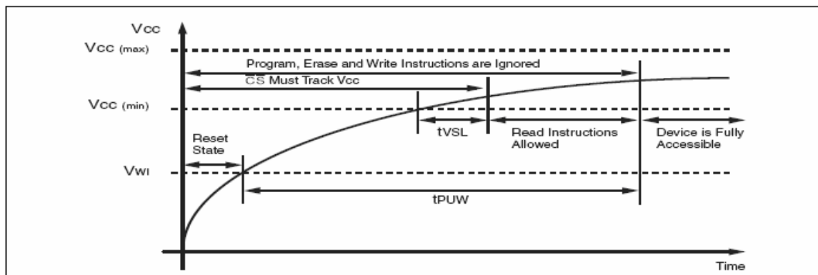
Figure 19. Power-up Timing
