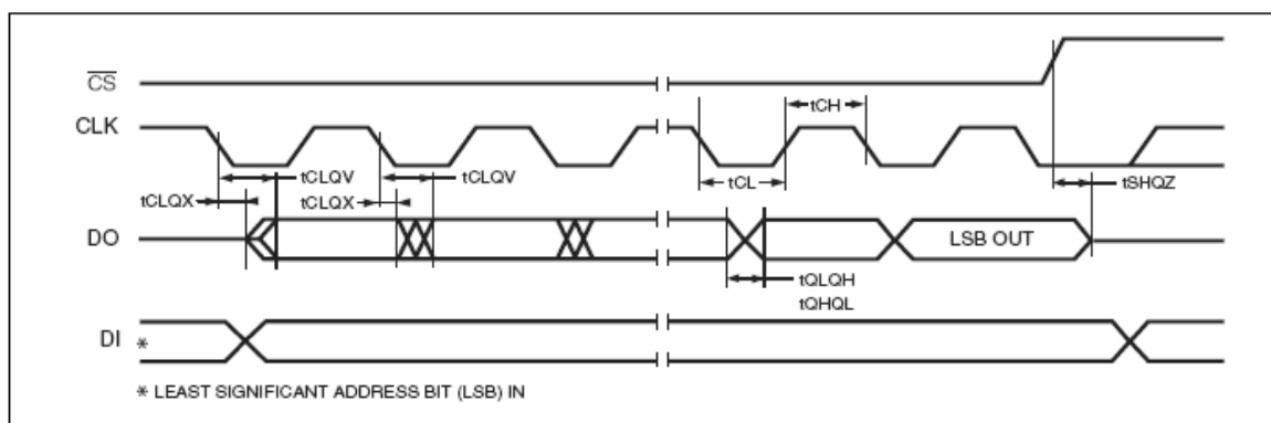
Figure 21. Serial Output Timing
