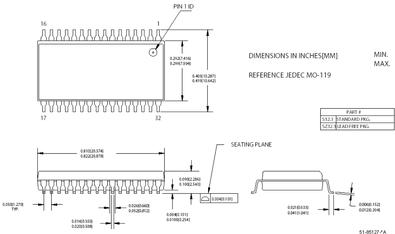
Figure 18. 32-Pin SOIC (51-85127)
