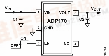
Figure 1. ADP170 with Fixed Output Voltage, 1.8 V
