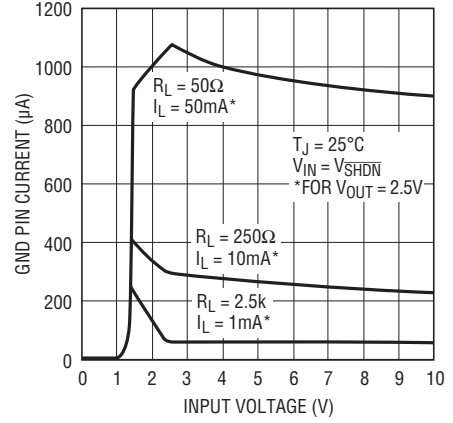
LT1763-2.5 GND Pin Current
