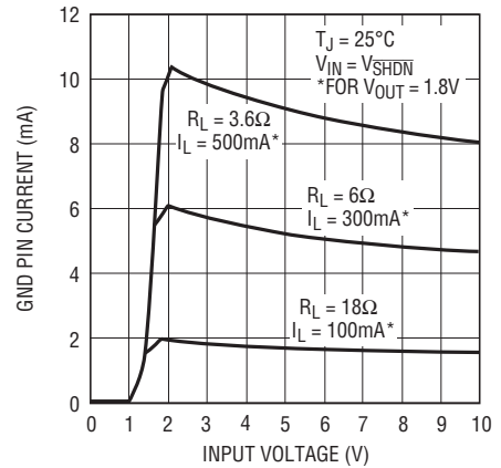
LT1763-1.8 GND Pin Current
