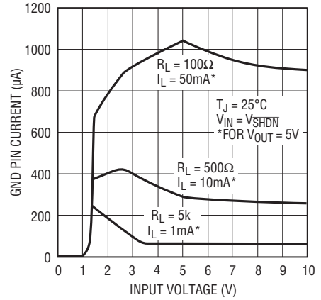
LT1763-5 GND Pin Current
