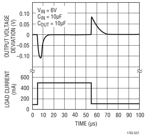
LT1763-5 Transient Response C_{BYP} = 0.01\mu F
