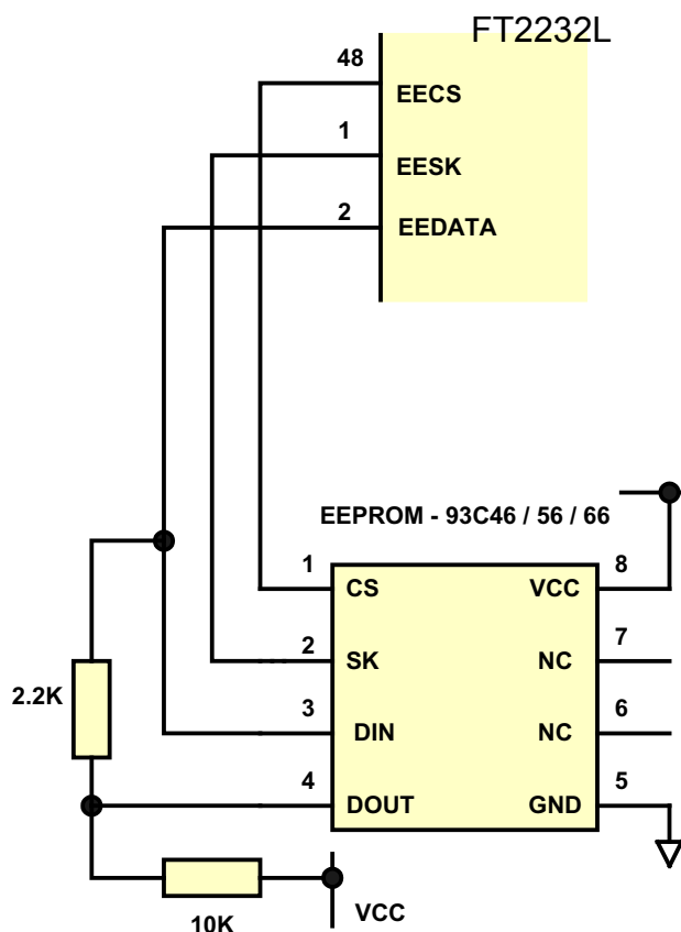
Figure 7 EEPROM Configuration
