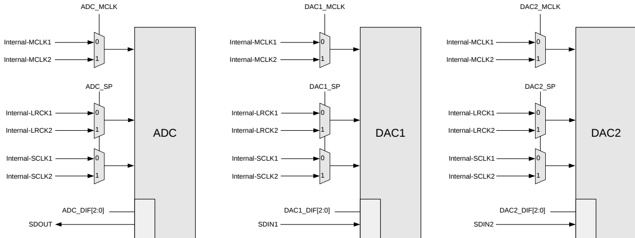
Figure 11. Converter Clocking
