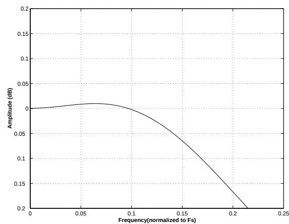
Figure 42. Quad-Speed Passband Ripple
