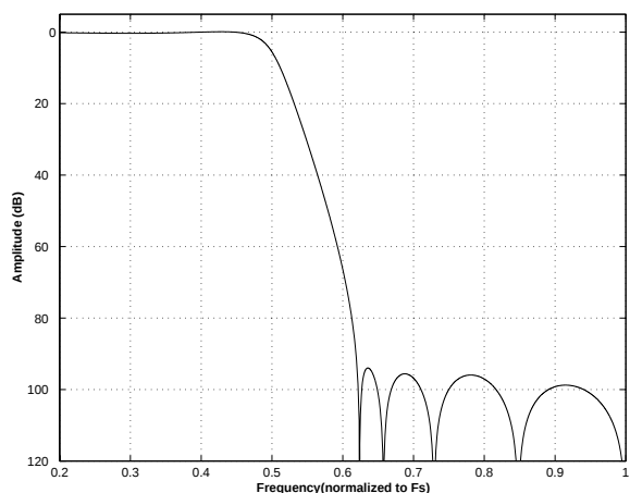
Figure 39. Quad-Speed Stopband Rejection
