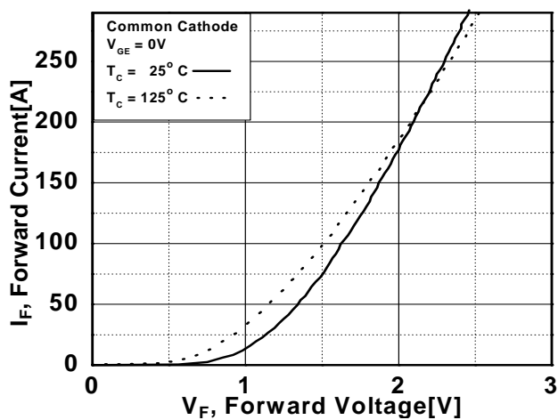
Fig 19. Forward Characteristics
