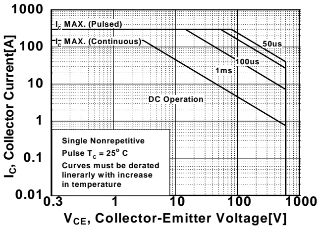
Fig 15. FBSOA Characteristics
