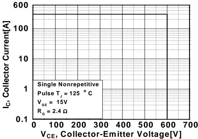
Fig 17. RBSOA Characteristics
