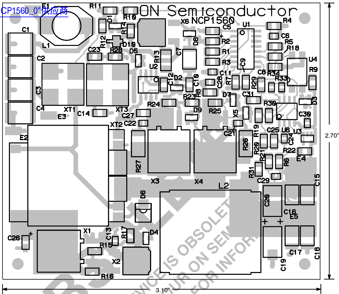
Figure 36. Board Arrangement
