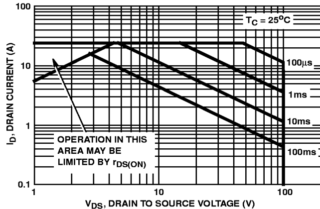
FIGURE 2. FORWARD BIAS SAFE OPERATING AREA
