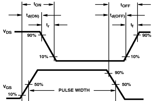
FIGURE 7. RESISTIVE SWITCHING WAVEFORMS
