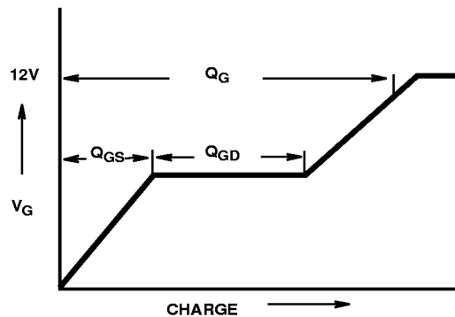
FIGURE 8. BASIC GATE CHARGE WAVEFORM
