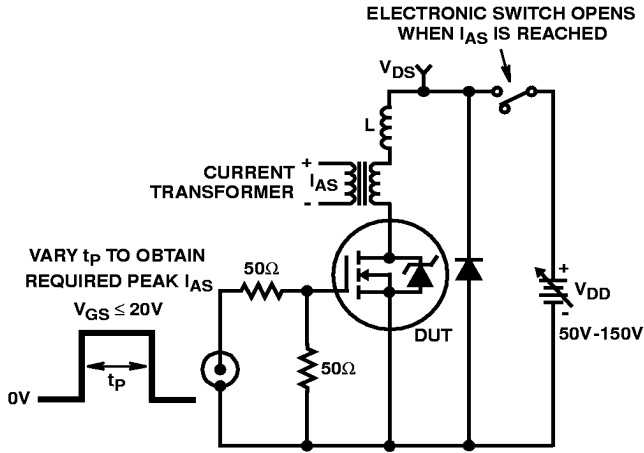
FIGURE 4. UNCLAMPED ENERGY TEST CIRCUIT
