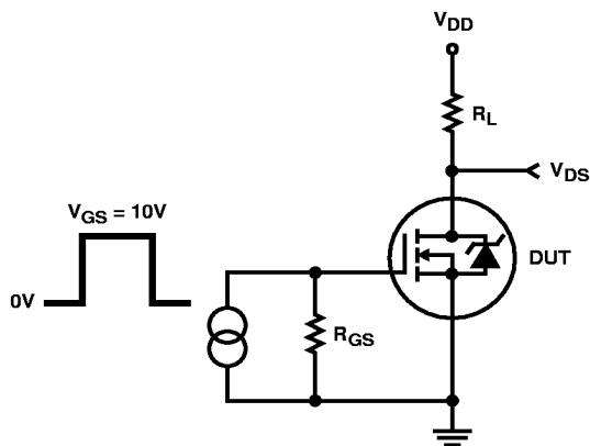
FIGURE 6. RESISTIVE SWITCHING TEST CIRCUIT
