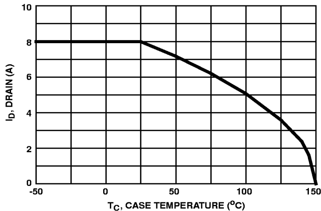
FIGURE 1. MAXIMUM CONTINUOUS DRAIN CURRENT vs CASE TEMPERATURE
