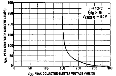
FIGURE 37 — MAXIMUM RATED REVERSE-BIAS SAFE OPERATING AREA (RBSOA)
