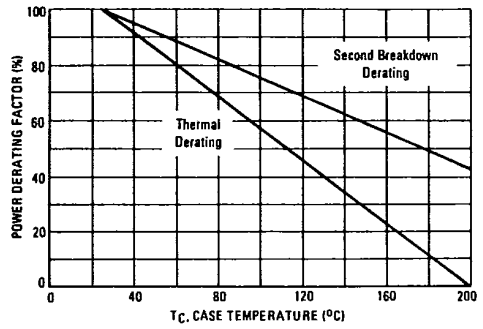
FIGURE 28 — POWER DERATING
