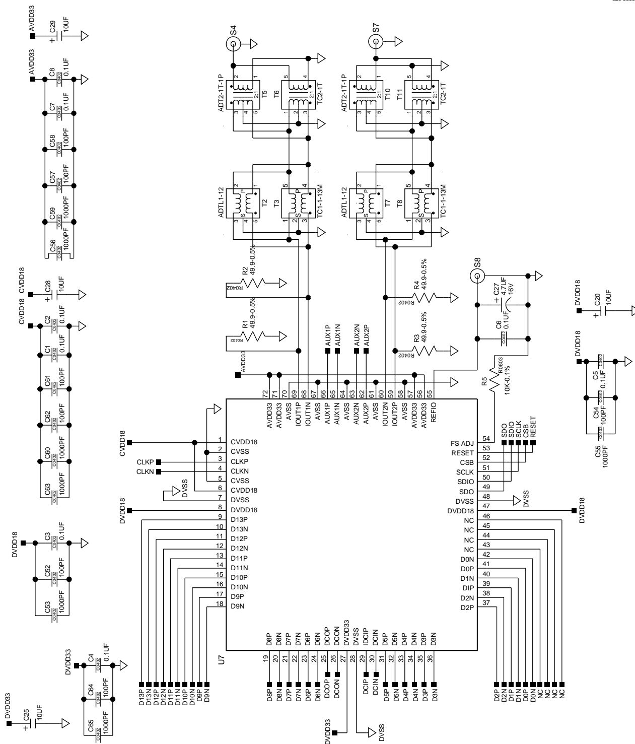
Figure 76. Main Schematic
