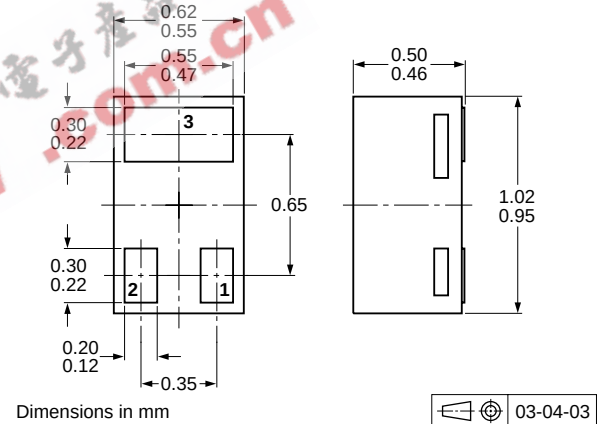
Fig 16. Package outline SOT883 (SC-101)
