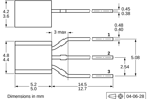
Fig 18. Package outline SOT54A
