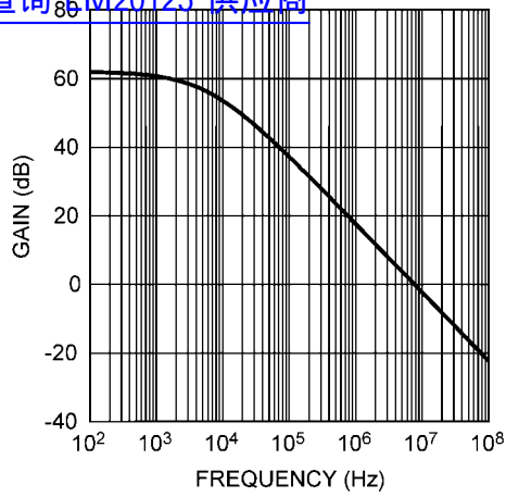
Error Amplifier Gain vs. Frequency 查询"LM20125"供应商
