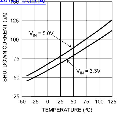
Shutdown Current vs. Temperature 查询"LM20125"供应商
