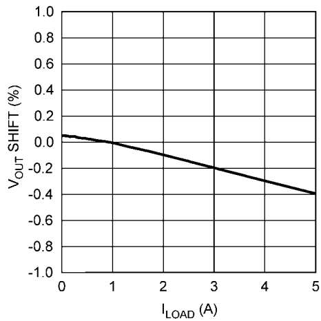
Load Regulation
