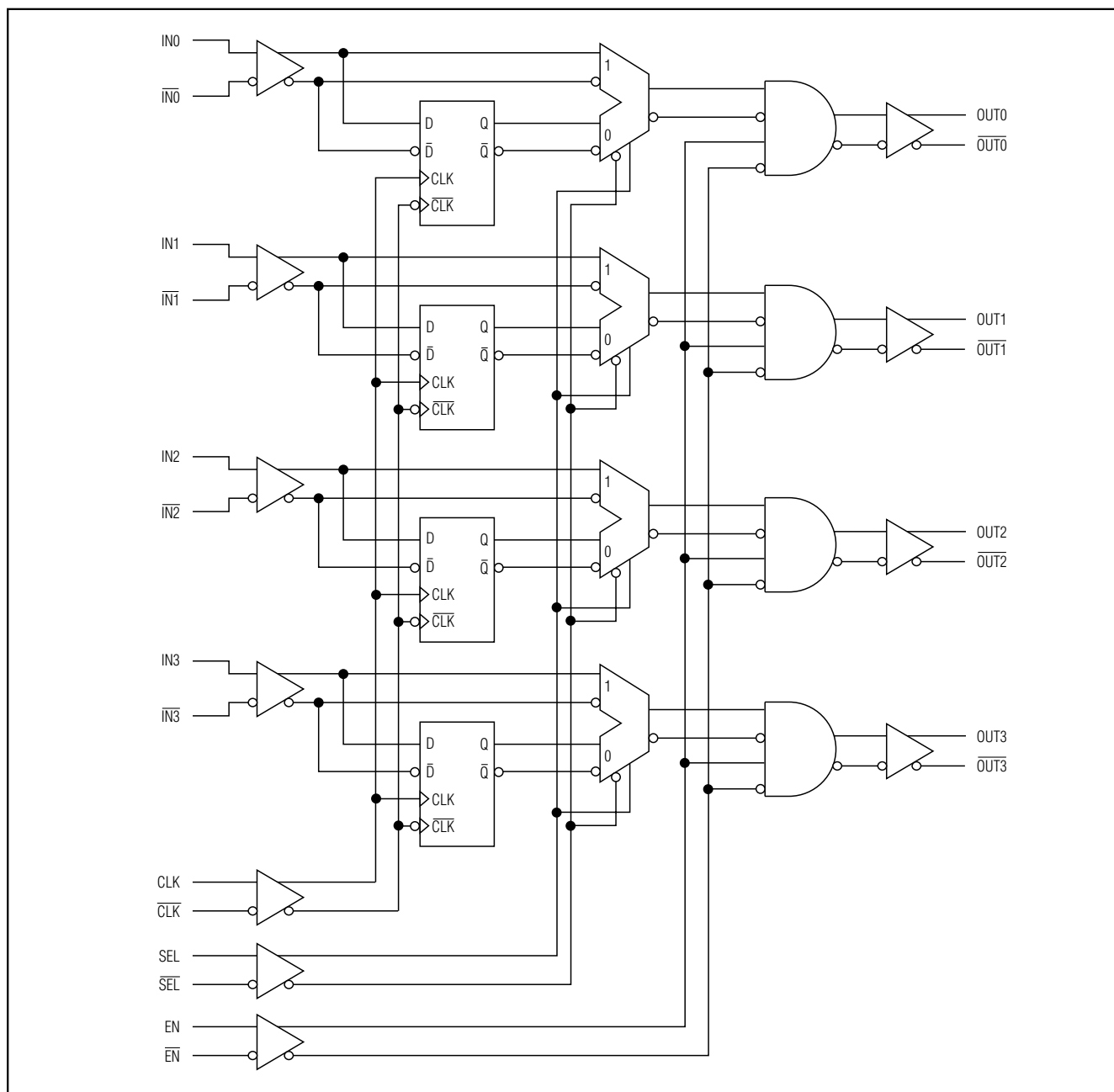
Functional Diagram
