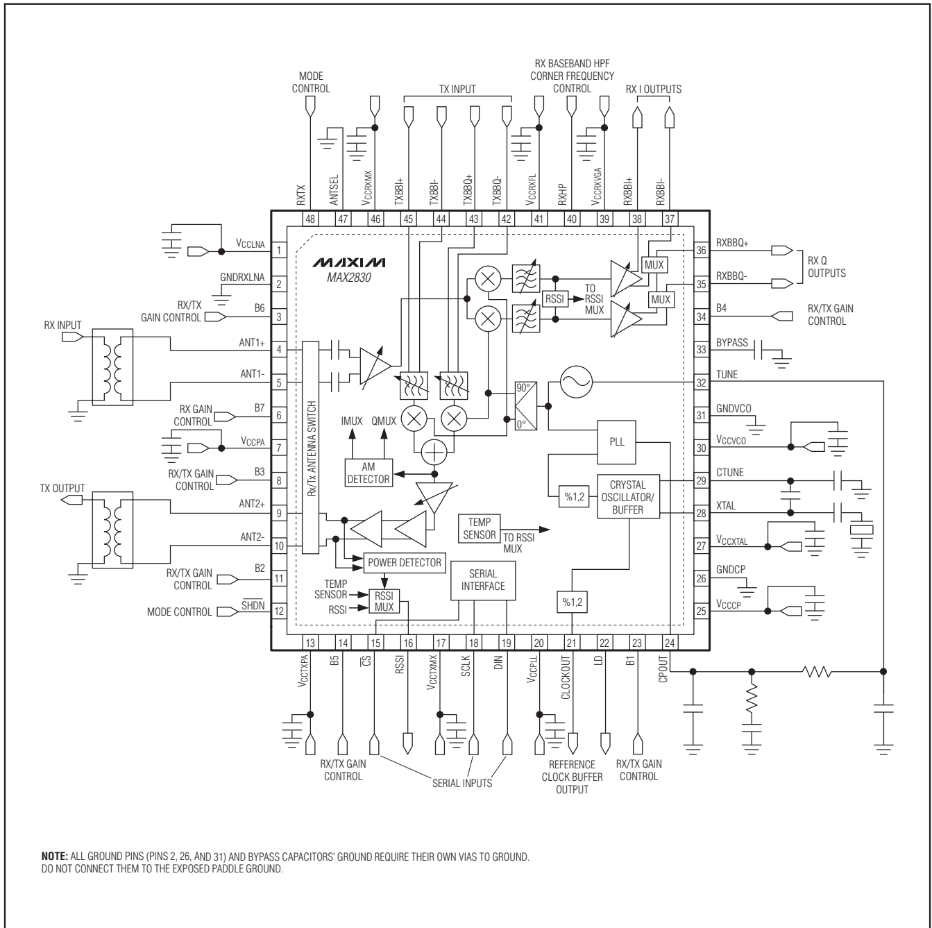
Block Diagram/Typical Operating Circuit
