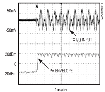
PA OUTPUT ENVELOPE RESPONSE
