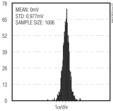
HISTOGRAM: Rx STATIC DC OFFSET
