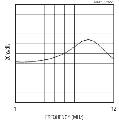
Rx BASEBAND FILTER GROUP DELAY
