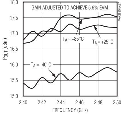
Tx OUTPUT POWER vs. FREQUENCY
