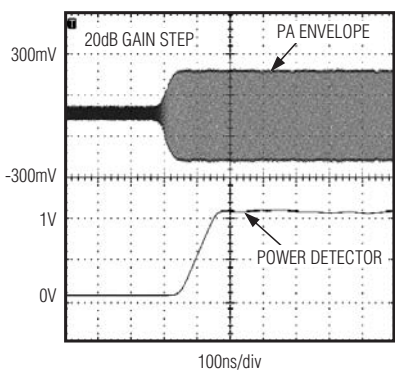
POWER-DETECTOR OUTPUT
