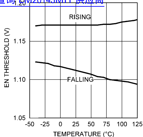
Enable Threshold vs. Temperature 查询"LM20143MH"供应商
