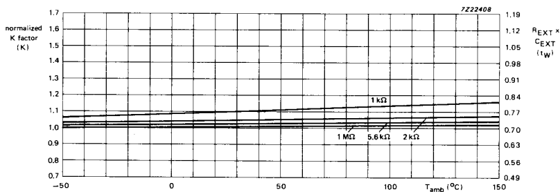
Fig. 18 Typical pulse width accuracy versus temperature; C_{EXT} = 1 \mu\text{F} ; V_{CC} = 4.5 \text{ V} .
