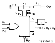
Fig. 4 Functional diagram.
