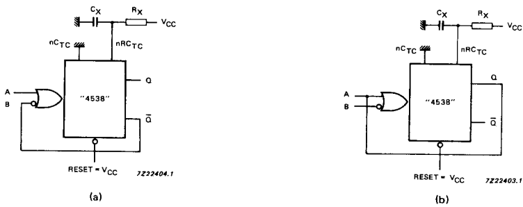
Fig. 10 Non-retriggerable monostable circuitry. (a) rising-edge triggered; (b) falling-edge triggered.
