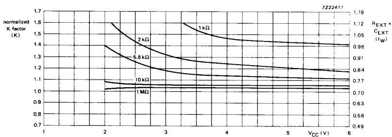
Fig. 15 Typical pulse width accuracy versus power supply; C_{EXT} = 1 \text{ nF} ; T_{amb} = 25^\circ \text{C} .
