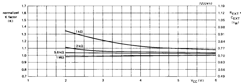
Fig. 16 Typical pulse width accuracy versus power supply; C_{EXT} = 100 \text{ nF} ; T_{amb} = 25^\circ \text{C} .
