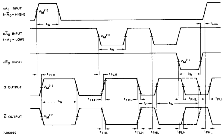
Fig. 8 Waveforms showing the input ( nA_1 , n\bar{A}_0 , n\bar{R}_D ) to output ( nQ , n\bar{Q} ) propagation delays, the output transition times, the input and output pulse widths, the removal time from direct reset ( n\bar{R}_D ) to input ( nA_1 , n\bar{A}_0 ), and the input retrigger time.
