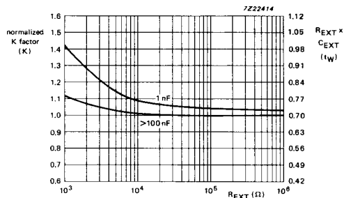
Fig. 13 Typical pulse width accuracy versus external resistance; V_{CC} = 4.5 \text{ V} ; T_{amb} = 25^\circ \text{C} .
