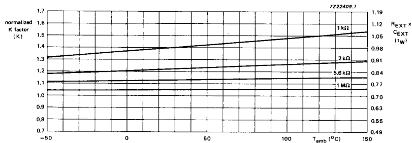
Fig. 17 Typical pulse width accuracy versus temperature; C_{EXT} = 1 \text{ nF} ; V_{CC} = 4.5 \text{ V} .
