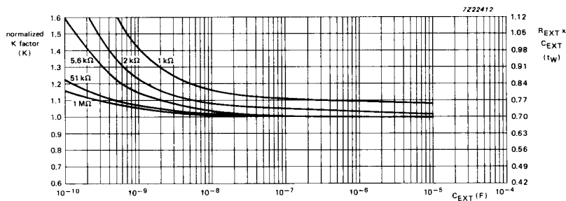
Fig. 12 Typical pulse width accuracy versus external capacitance; V_{CC} = 4.5 \text{ V} ; T_{amb} = 25^\circ \text{C} .
