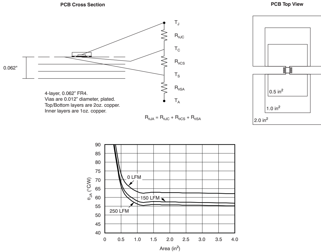
Figure 30. DRC (3 x 3 SON) PCB Layout and Corresponding R_{thJA} Data, Top Layer Only
