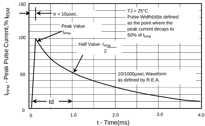
Fig.3 - Pulse Waveform
